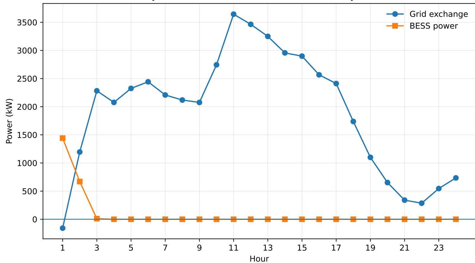
Representative 24-h Grid and BESS Dispatch
