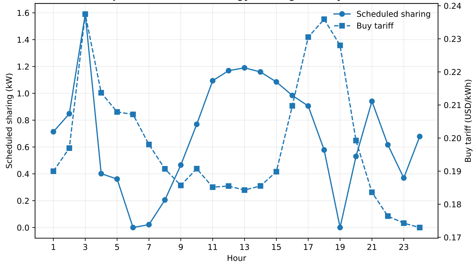
Representative 24-h Energy Sharing and Buy Tariff
