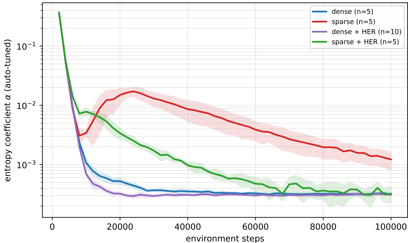
FetchReach-v3: SAC entropy coefficient over training
