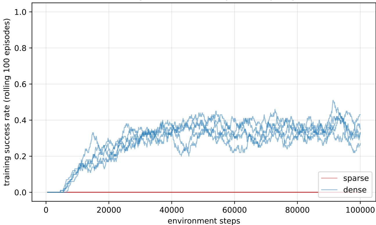
Training-time success (exploration policy)
