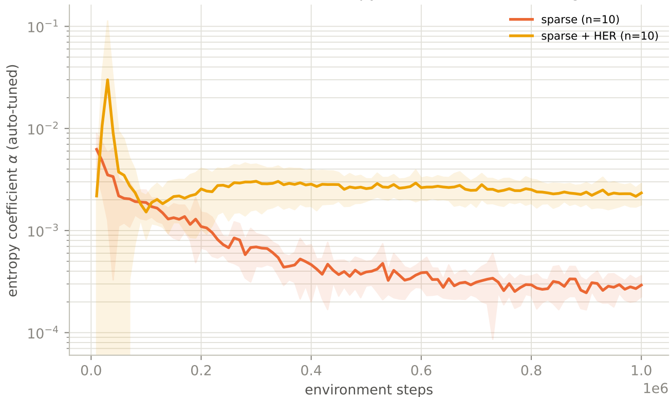
FetchPush-v3: SAC entropy coefficient over training
