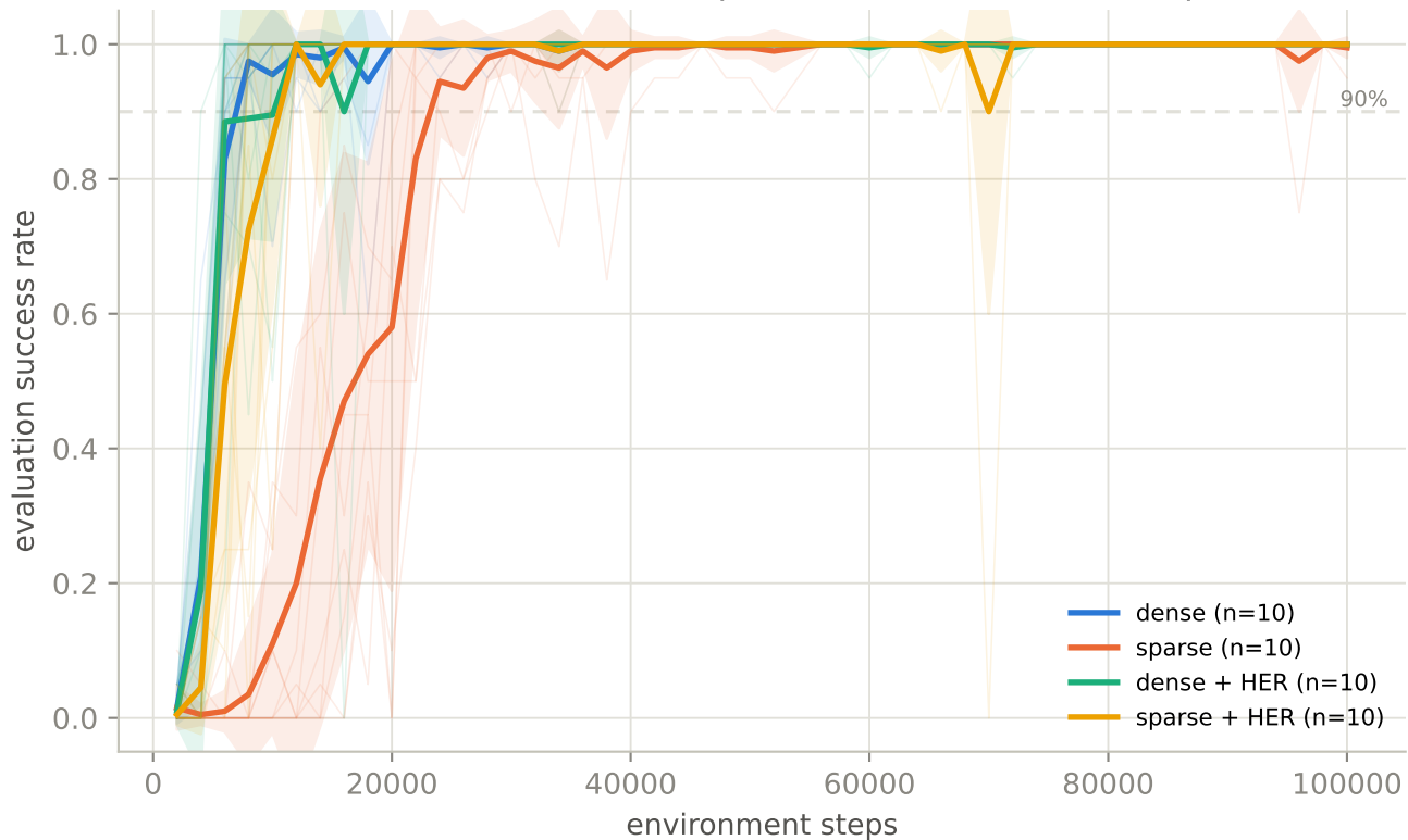
SAC on FetchReach-v3: dense vs sparse vs dense + HER vs sparse + HER
