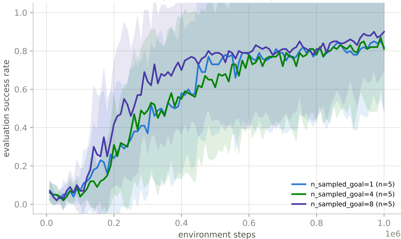
FetchPush-v3 sparse+HER: relabeling-ratio ablation
