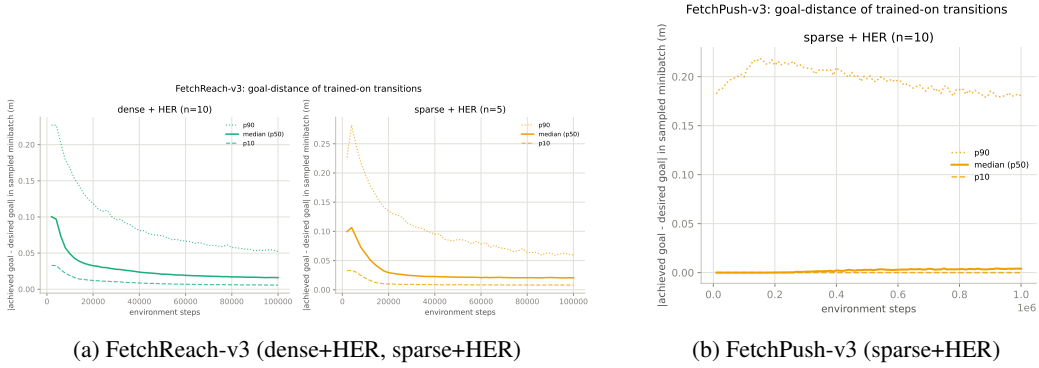
Figure 3: The p_{10} , median ( p_{50} ), and p_{90} of \|\text{achieved goal} - \text{desired goal}\| across transitions sampled for training. The three percentiles are shown as separate lines rather than as a shaded band so that changes in the upper tail remain visible when the median is close to zero.
