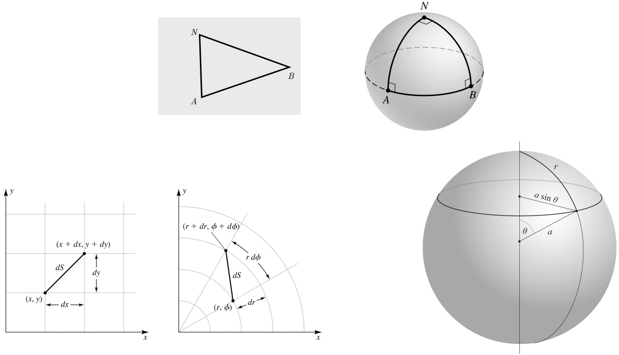
Figure 2.1: Top panel (right): The sum of the interior angles of a triangle ABN on a 2-sphere is > \pi , in this particular case it is 3\pi/2 . On the plane it is of course \pi . Bottom Panel (right): The circumference of the circle of radius r is < 2\pi r , it is C = 2\pi r \sin(r/a)/(r/a) . On a plane it would be C = 2\pi r . Bottom Panel (left): Cartesian and Polar co-ordinates in a 2D plane.
