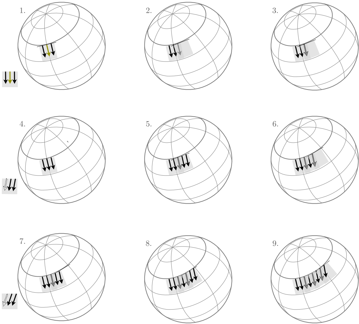
Figure 3.1: Parallel transport on a sphere using post-it” notes. 1. Draw three arrows perpendicular to the sticky upper edge of a post-it note on a flat surface. Stick this note on a globe, such that the upper edge of the post-it note is tangent to a latitude. The middle arrow is tangent to a longitude. 2. Take another post-it note and stick it again on the globe. The second note’s upper edge is also tangent to the same latitude, but at a different longitude. Make sure the two notes overlap a bit. 3. Trace out the last arrow of note 1 onto note 2. 4. Remove the note in 3, put it on a flat surface and draw arrows parallel to the traced-out arrow. The arrows are locally parallel. 5. Put the note in 4 back on the sphere in the same way as in 3. For sufficiently small post-it notes, this gives a discrete approximation to parallel transport from one tangent plane to the next. 6. Repeat 3 with a new note. 7. Repeat step 4, but with the note in 6. 8. Stick the note from 7 back on the sphere as it was in 6. At the most nearby longitude shown, the last arrow is no longer perpendicular to the latitude. Equivalently, it is not tangent to its local longitude. 9. Continue the steps to see the rotation” continue!
