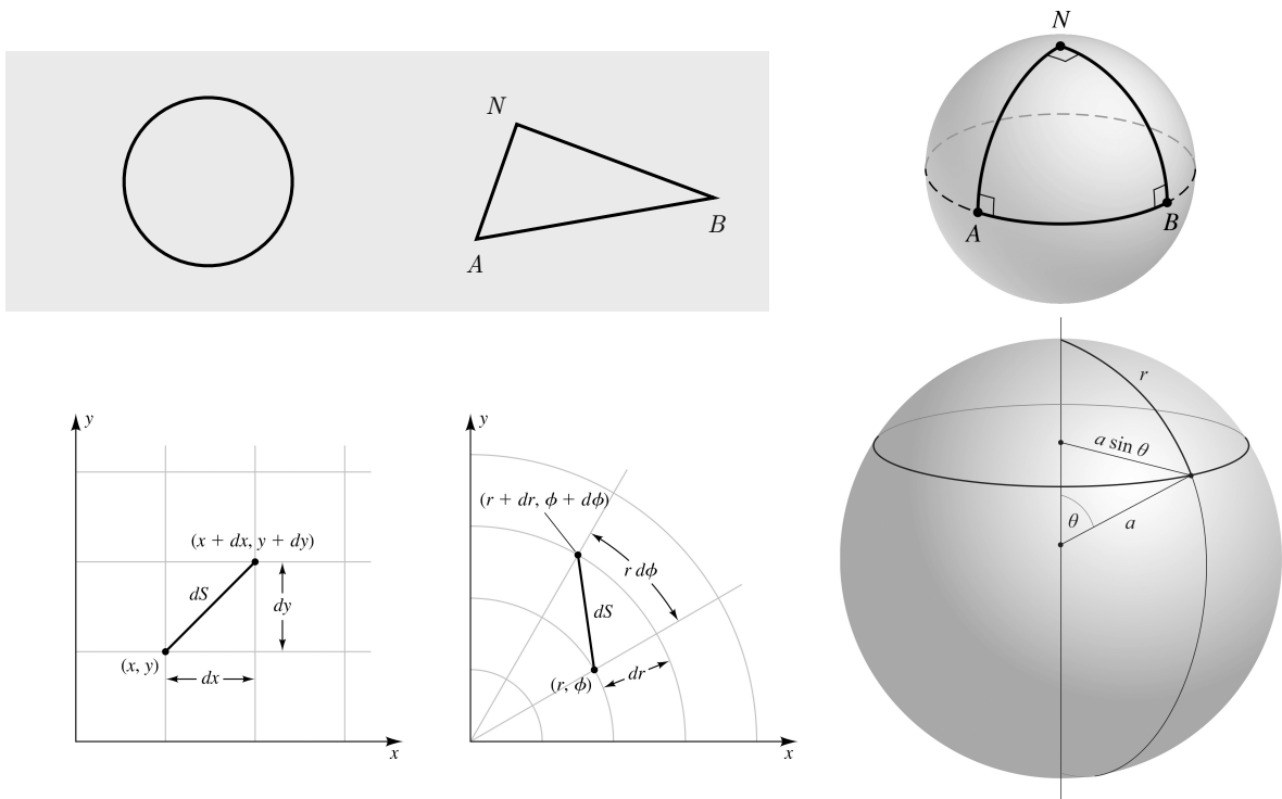
Figure 2.1: Top panel (right): The sum of the interior angles of a triangle ABN on a 2-sphere is > \pi , in this particular case it is 3\pi/2 . On the plane it is of course \pi . Bottom right: The circumference of the circle of radius r is < 2\pi r , it is C = 2\pi r \sin(r/a)/(r/a) (bottom right). On a plane it would be C = 2\pi r . Bottom Left: Cartesian and Polar co-ordinates in a 2D plane. Bottom Right: r and \theta co-ordinates on the sphere. Part of the Fig. adapted from Hartle.
