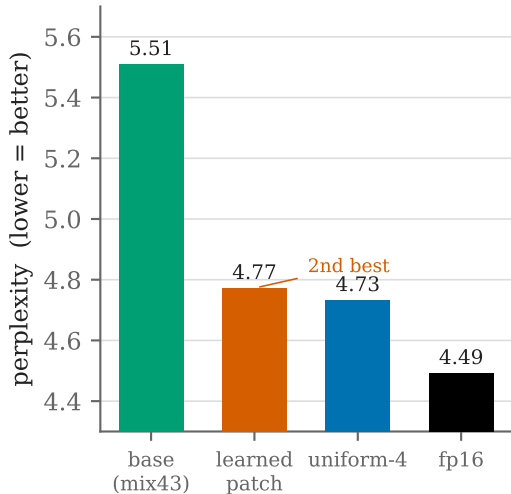
what perplexity says
