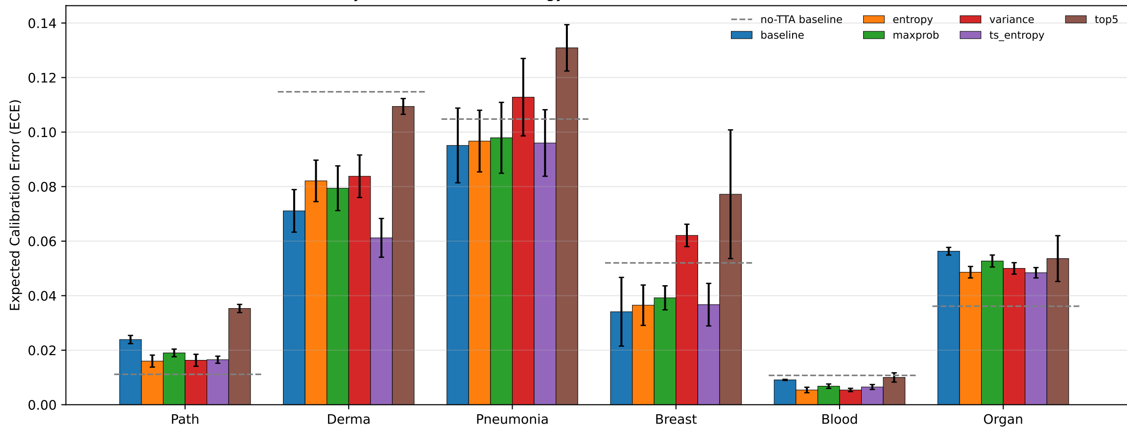
ECE by dataset and TTA strategy — ResNet-18 (mean \pm std over 3 seeds)
