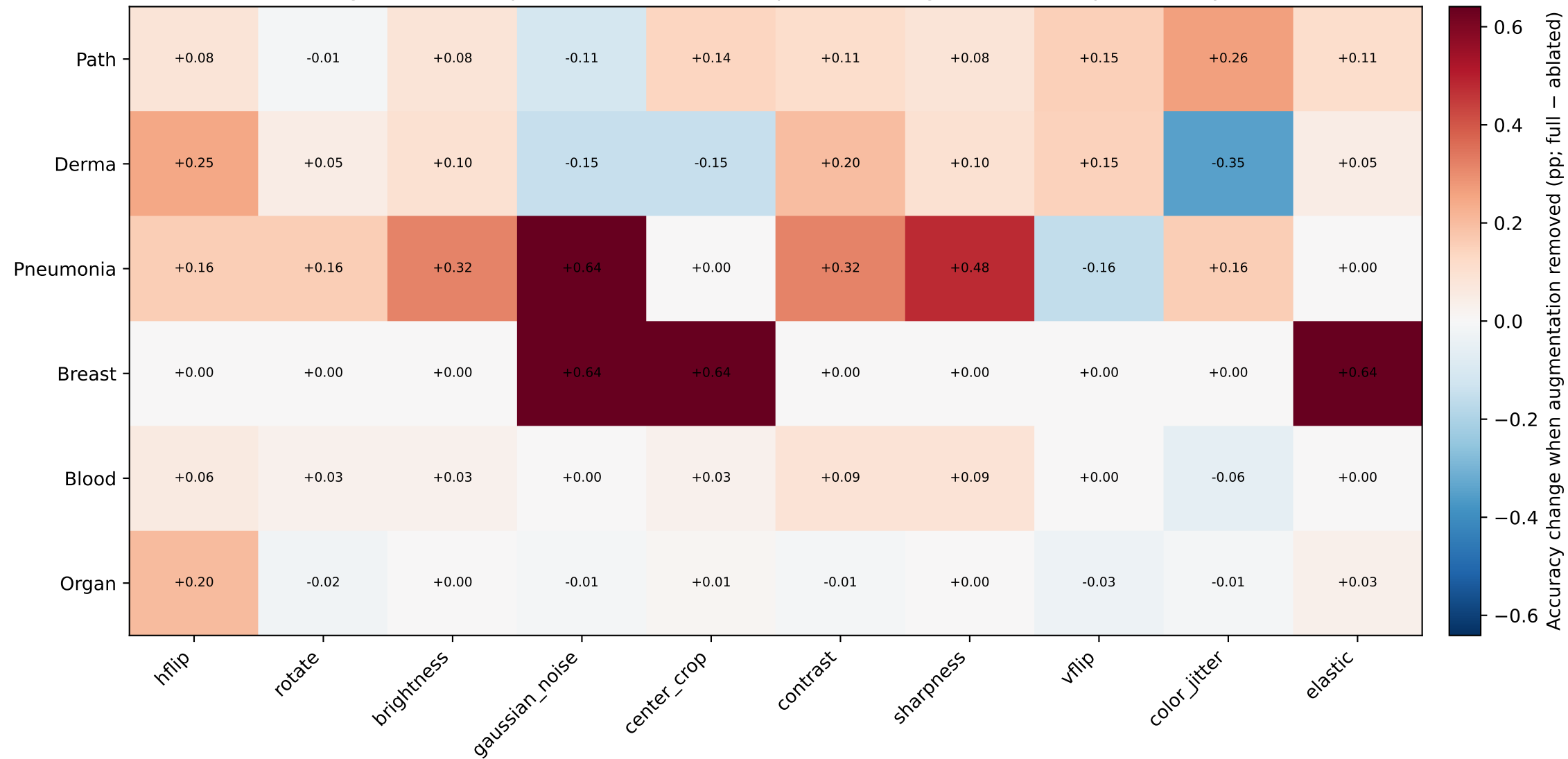
Augmentation importance — ResNet-18 (positive = augmentation helps accuracy)
