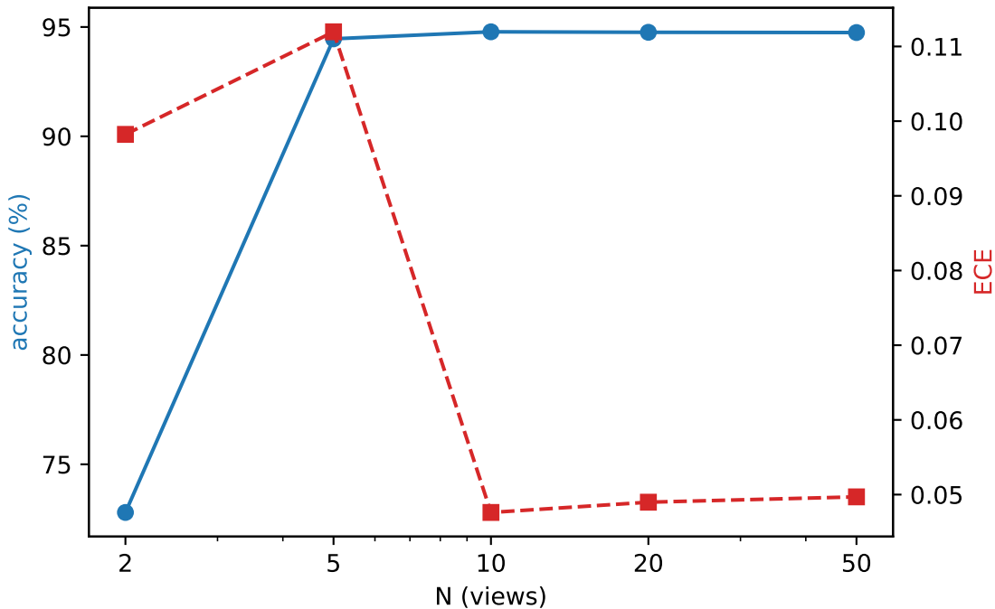
organamnist — variance: accuracy & ECE vs N
