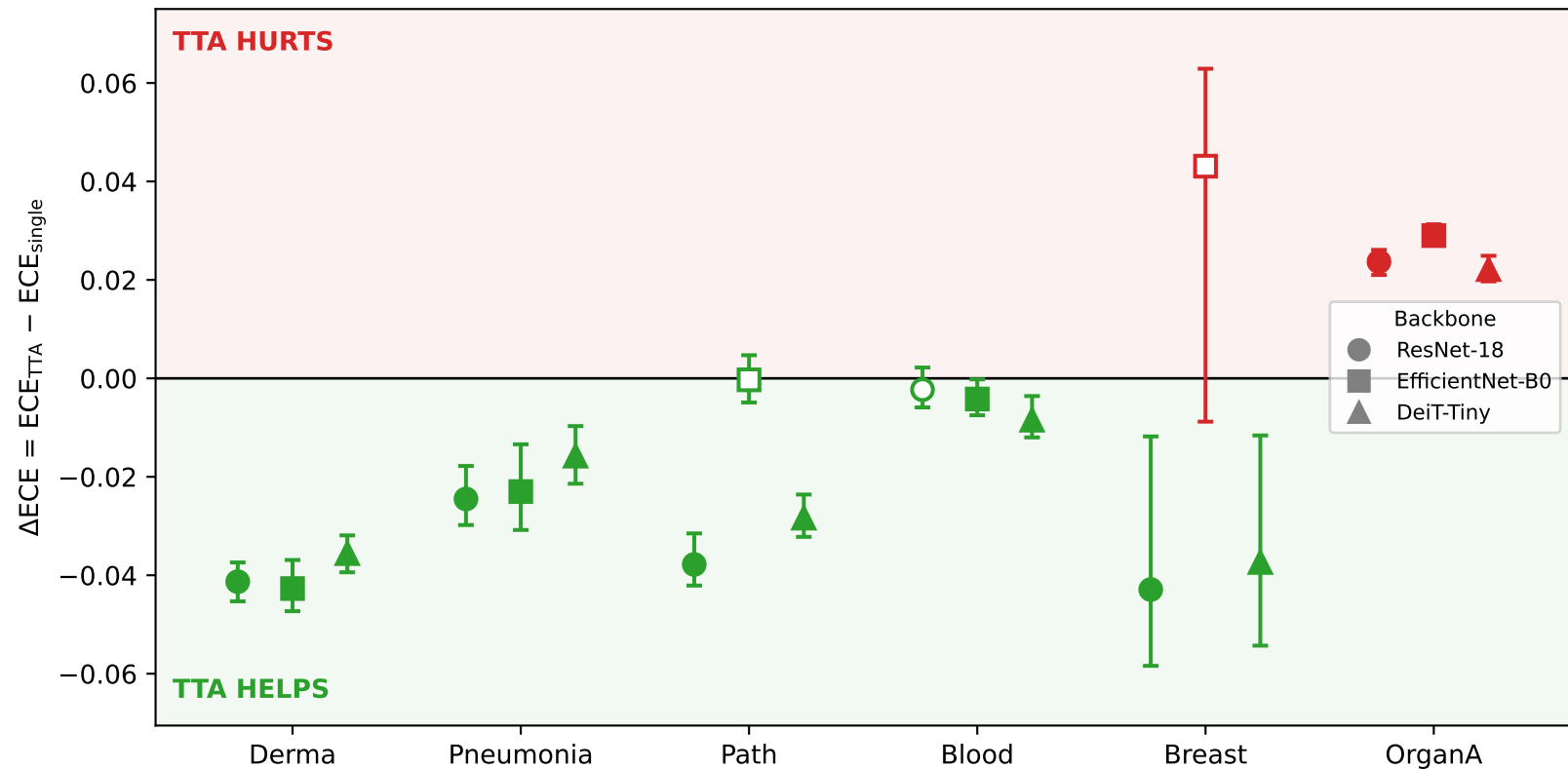
Sign-flip test: does equal-weight TTA help or hurt calibration? paired bootstrap, 95% CI (filled marker = CI excludes 0)
