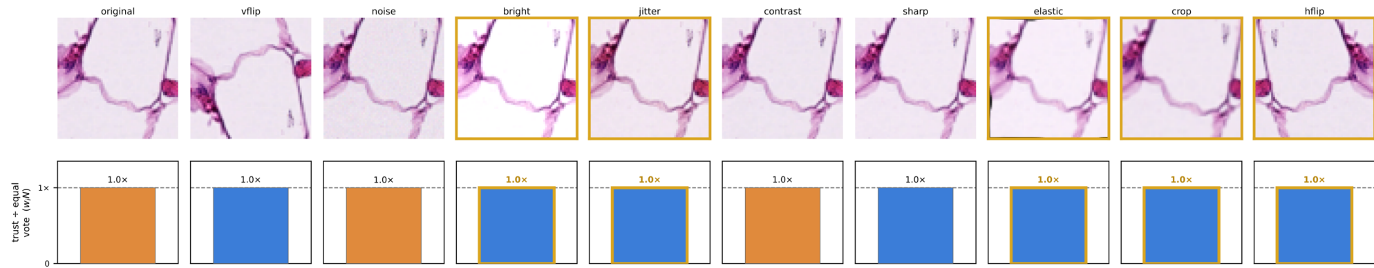
Figure 1 (EfficientNet-B0), sample 5
