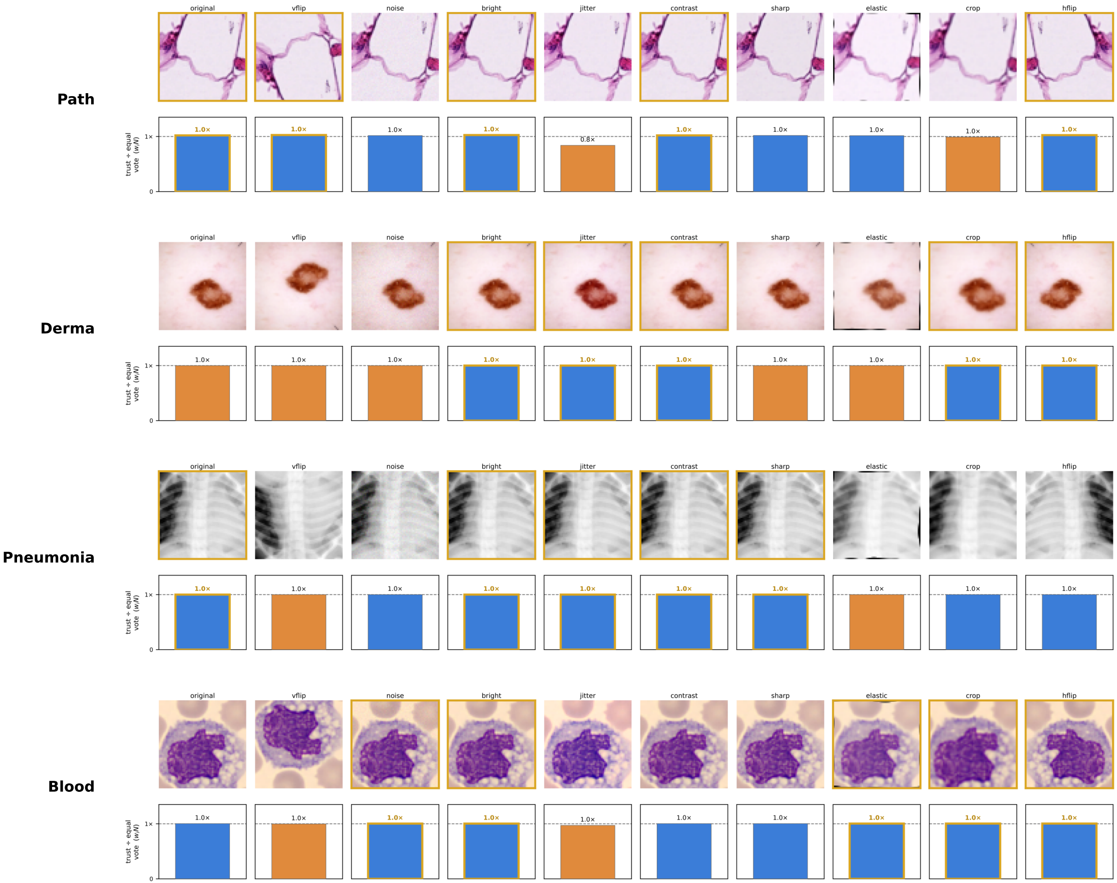
Figure 1 (ResNet-18), sample 5
