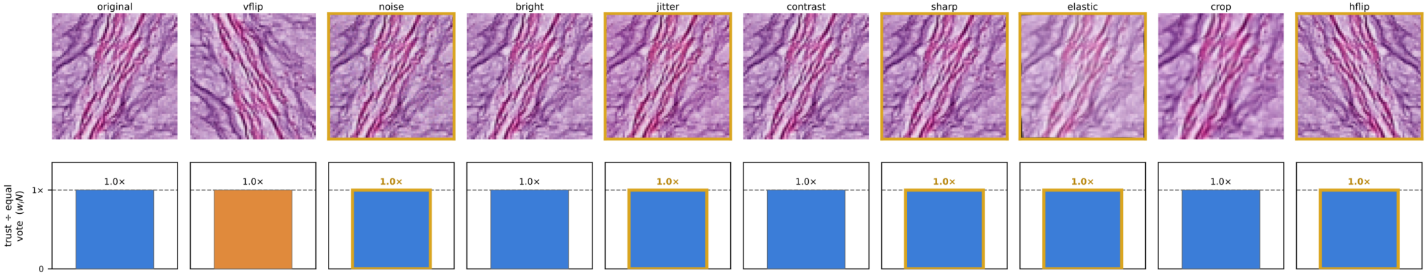
Path sample 3
