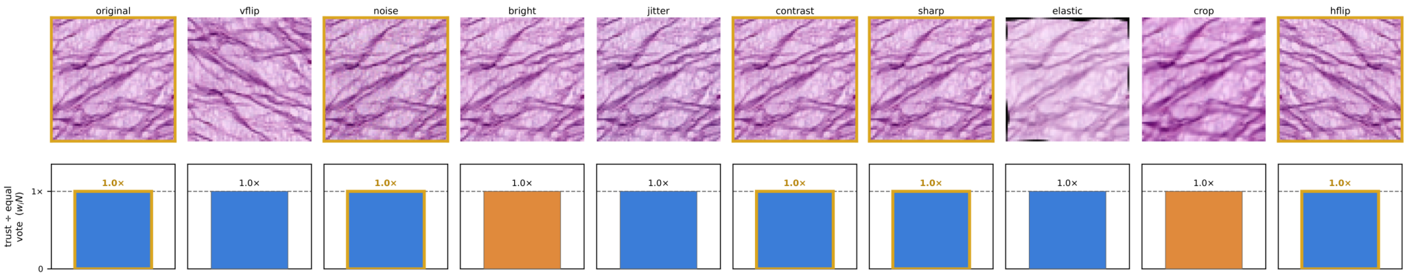
Path sample 6
