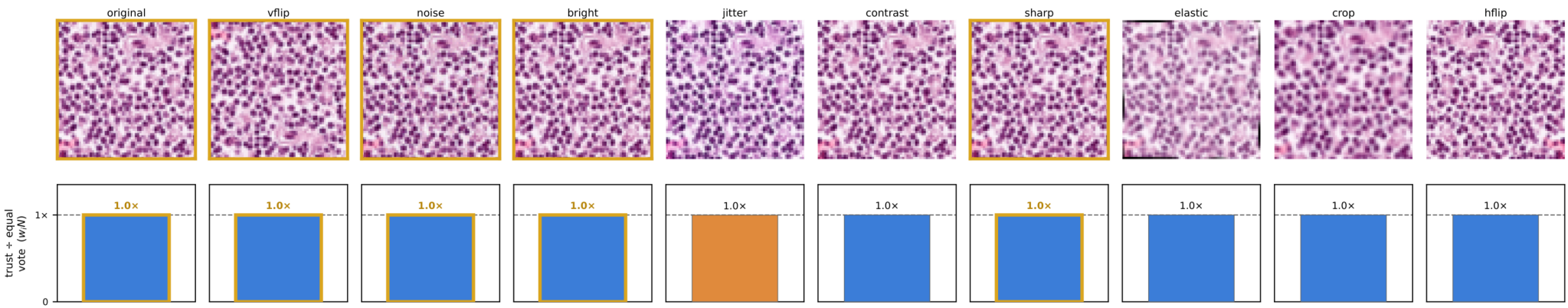
Path sample 1
