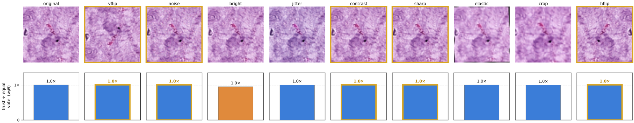
Path sample 2
