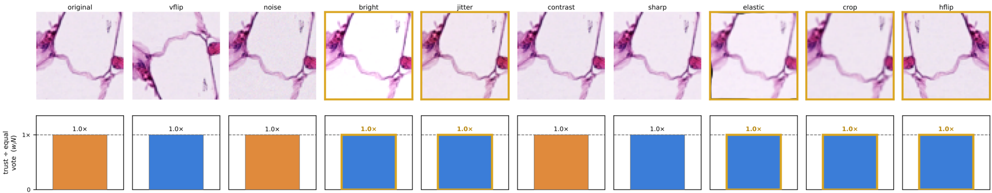
Path sample 5
