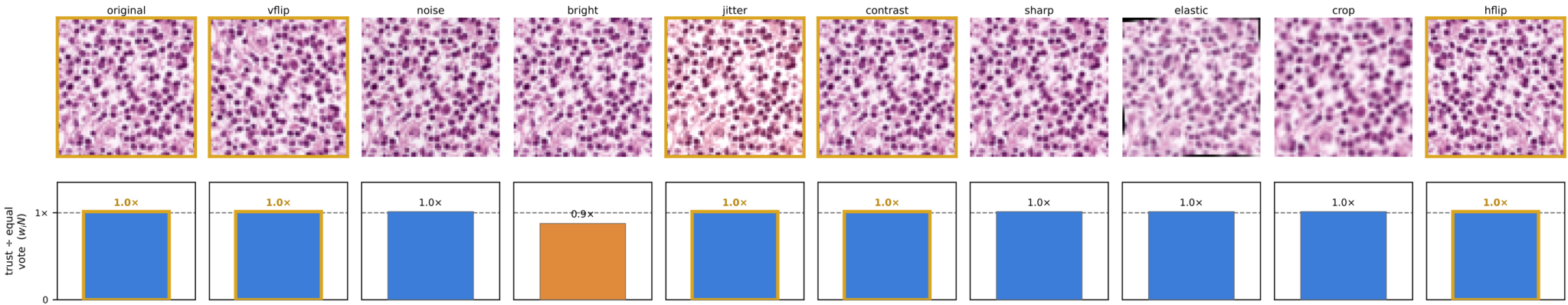
Path sample 4
