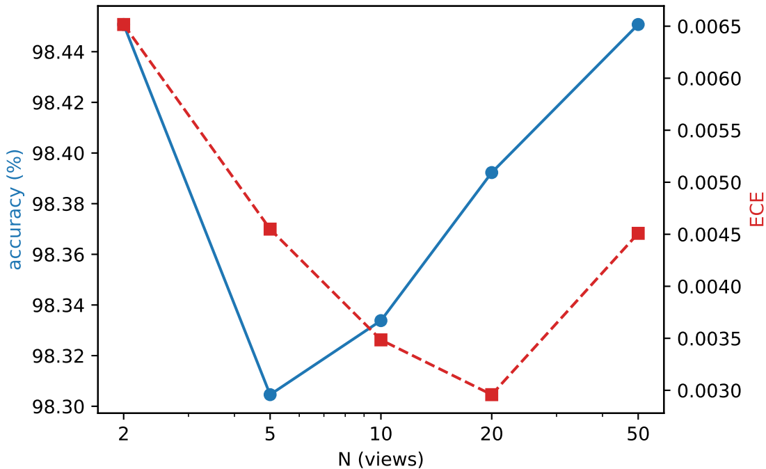
bloodmnist — entropy: accuracy & ECE vs N
