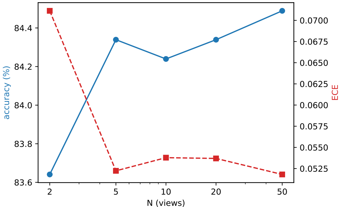
dermamnist — entropy: accuracy & ECE vs N
