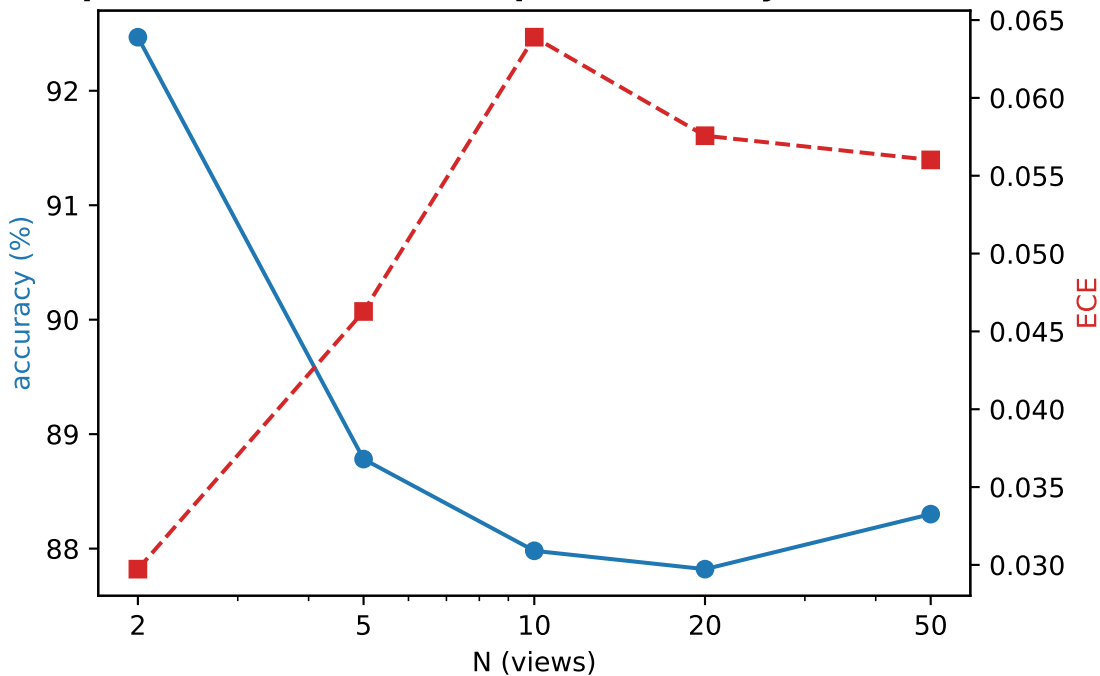
pneumoniarnnist — maxprob: accuracy & ECE vs N
