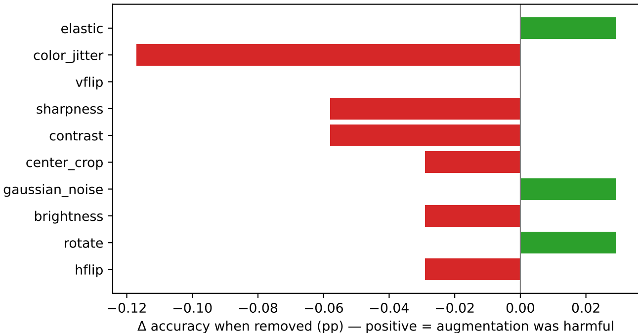
bloodmnist — entropy: leave-one-out
