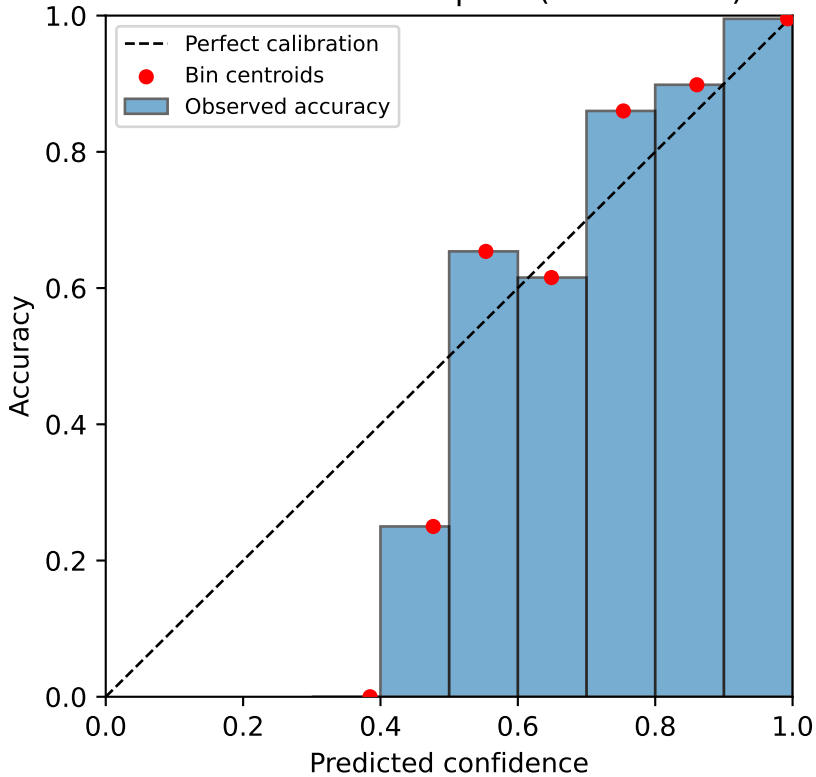
bloodmnist — maxprob (ECE=0.007)
