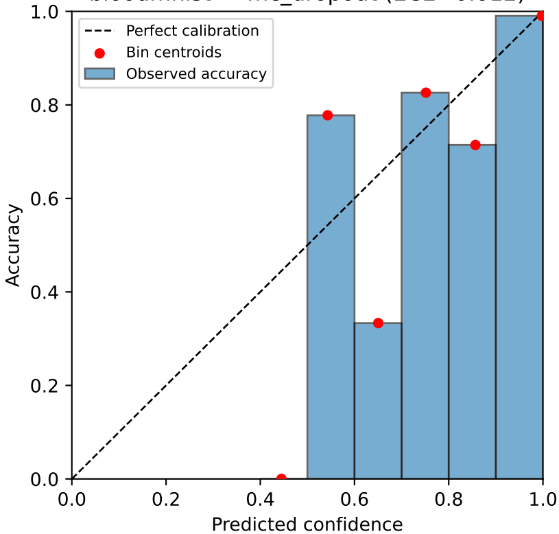
bloodmnist — mc_dropout (ECE=0.012)
