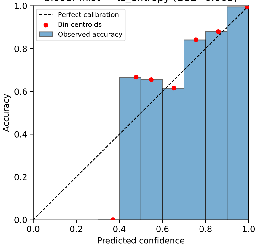
bloodmnist — ts_entropy (ECE=0.005)
