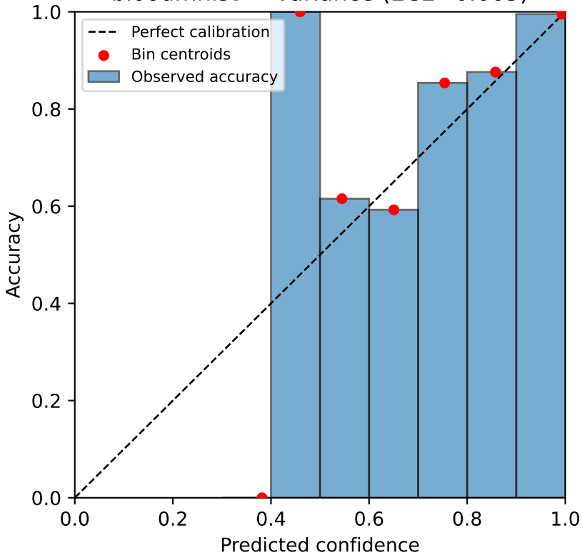
bloodmnist — variance (ECE=0.005)
