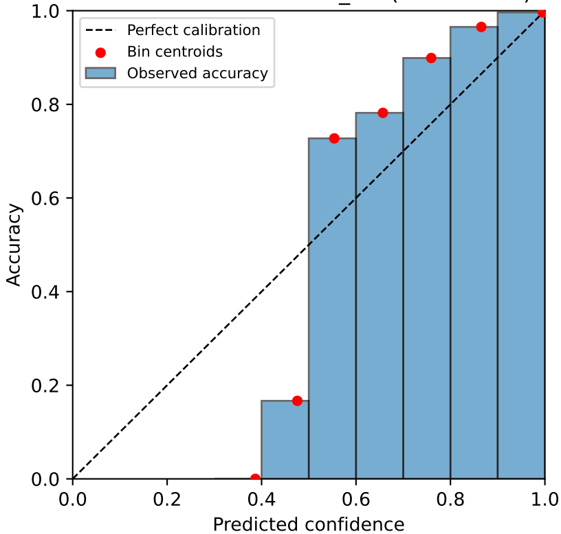
bloodmnist — variance_inv (ECE=0.017)
