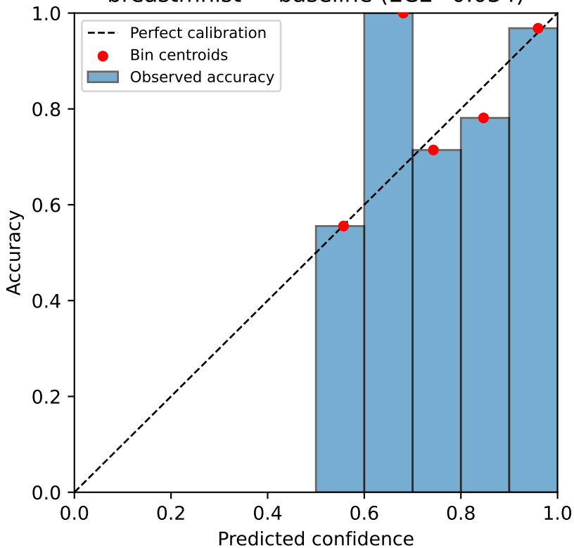
breastmnist — baseline (ECE=0.034)
