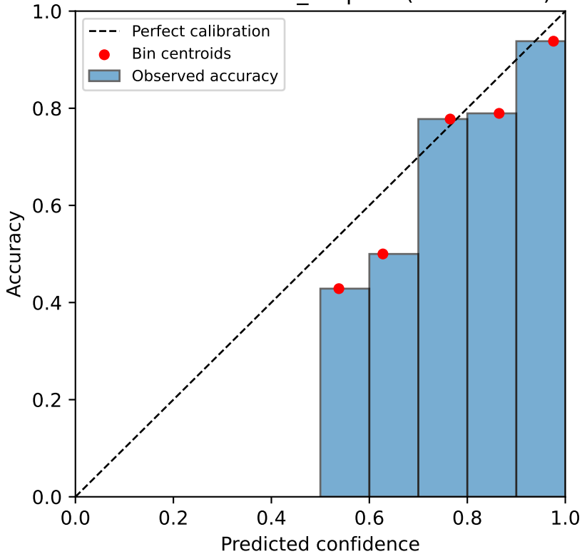
breastmnist — mc_dropout (ECE=0.049)
