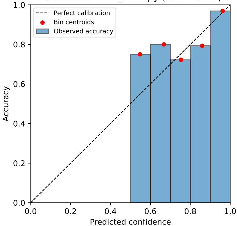
breastmnist — ts_entropy (ECE=0.035)
