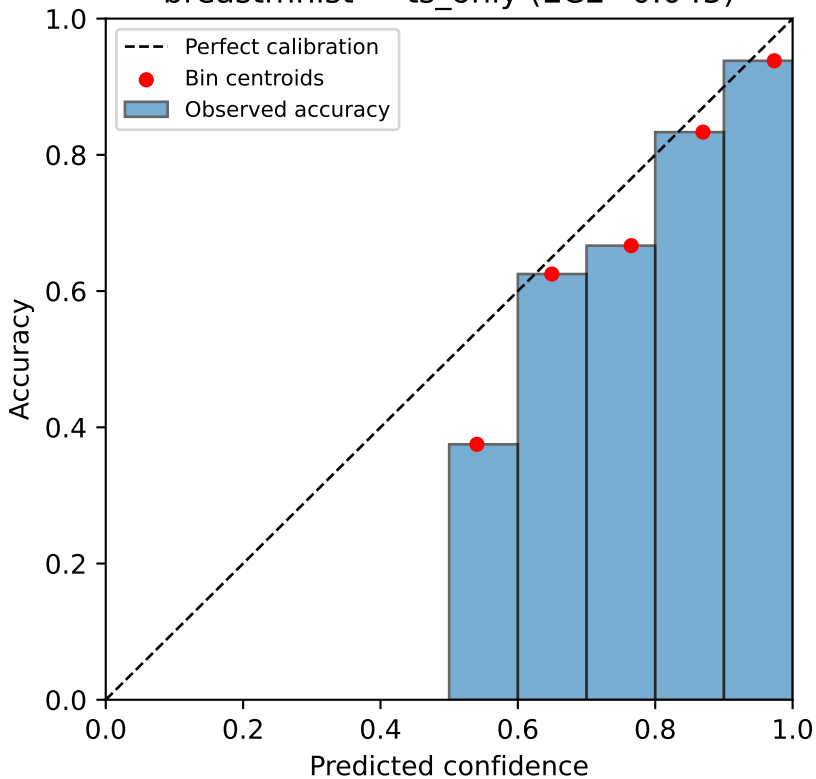
breastmnist — ts_only (ECE=0.045)
