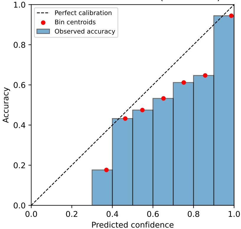
dermannist — baseline (ECE=0.071)
