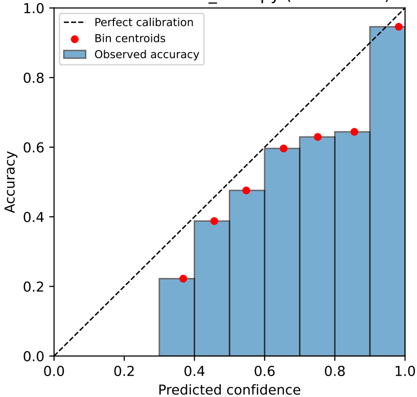
dermannist — ts_entropy (ECE=0.063)
