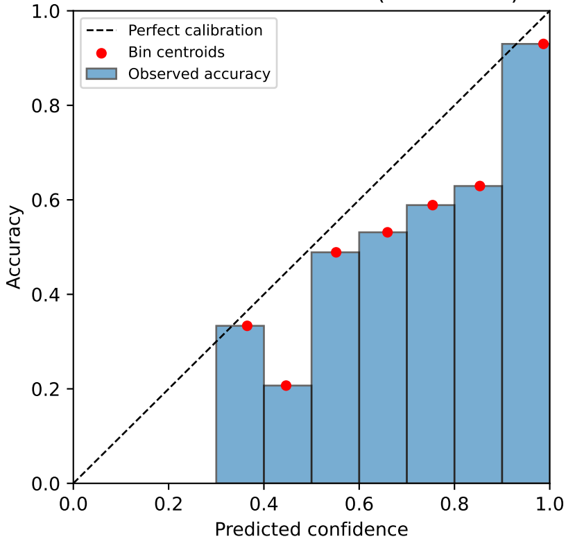
dermamnist — variance (ECE=0.084)
