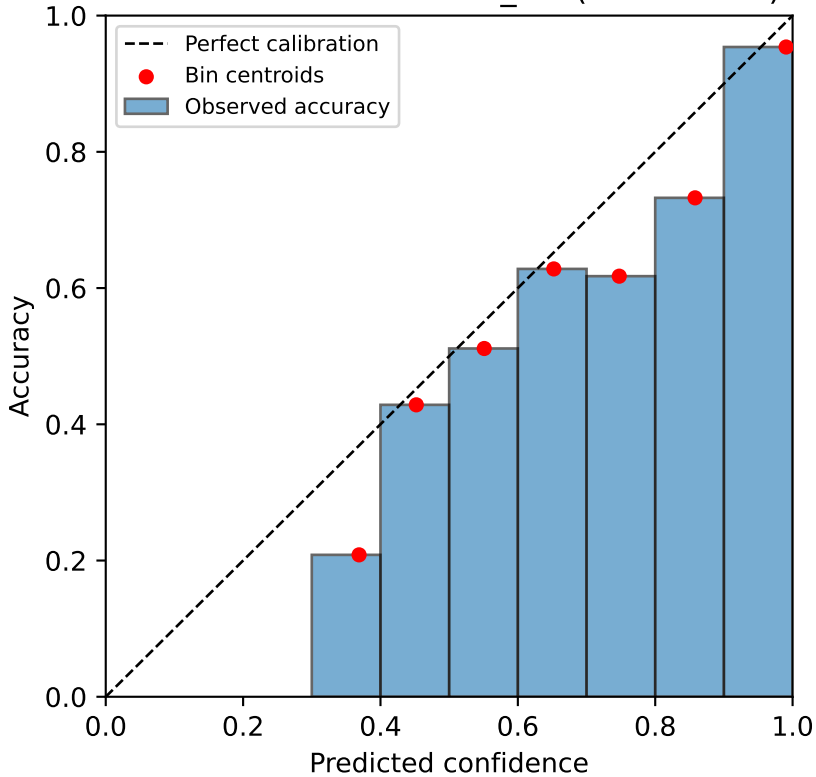
dermamnist — variance_inv (ECE=0.054)
