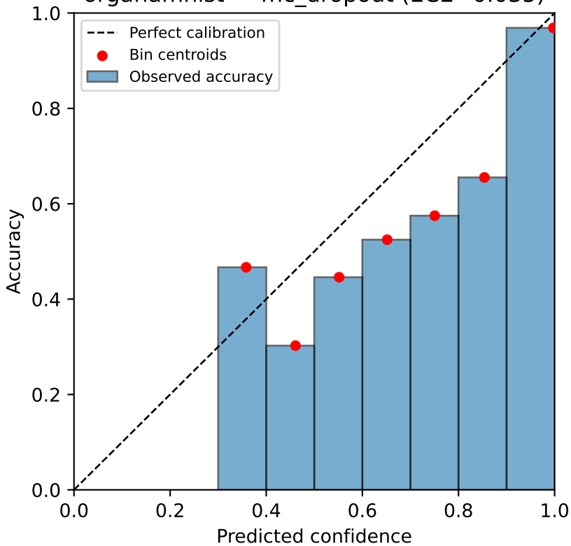
organamnist — mc_dropout (ECE=0.035)
