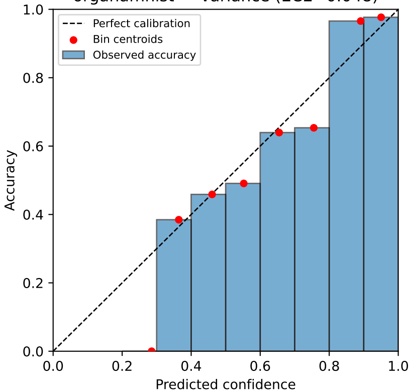
organamnist — variance (ECE=0.048)
