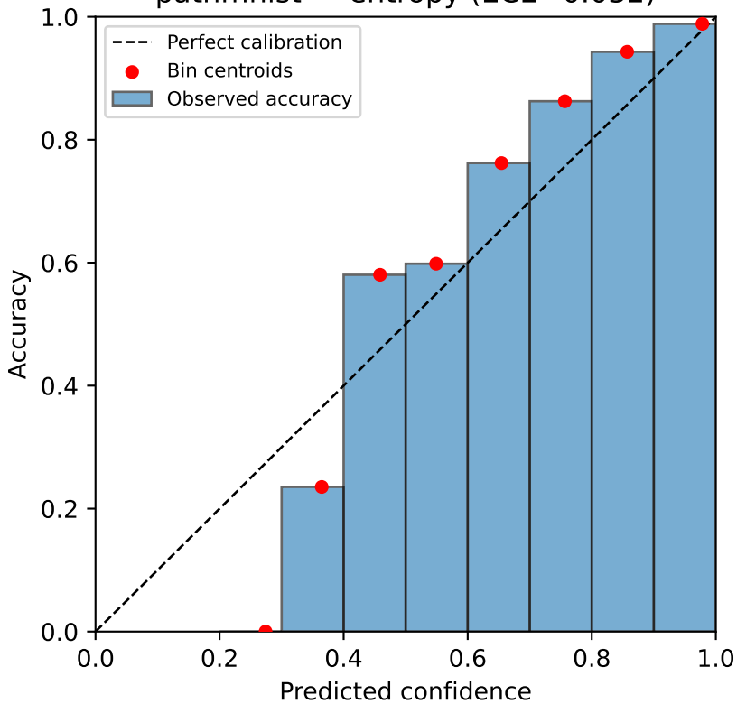
pathmnist — entropy (ECE=0.032)
