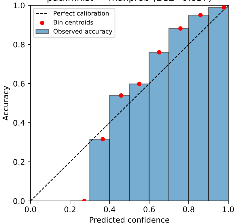
pathmnist — maxprob (ECE=0.037)
