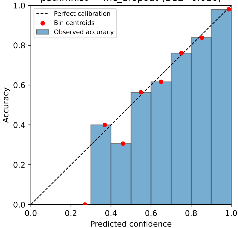
pathmnist — mc_dropout (ECE=0.010)
