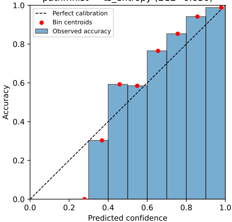
pathmnist — ts_entropy (ECE=0.030)
