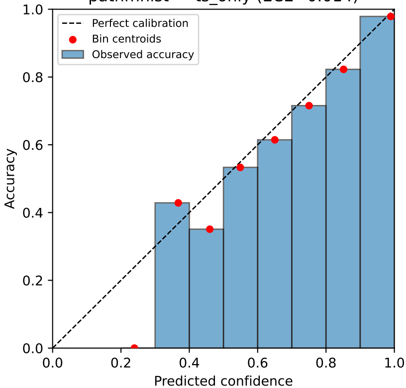
pathmnist — ts_only (ECE=0.014)
