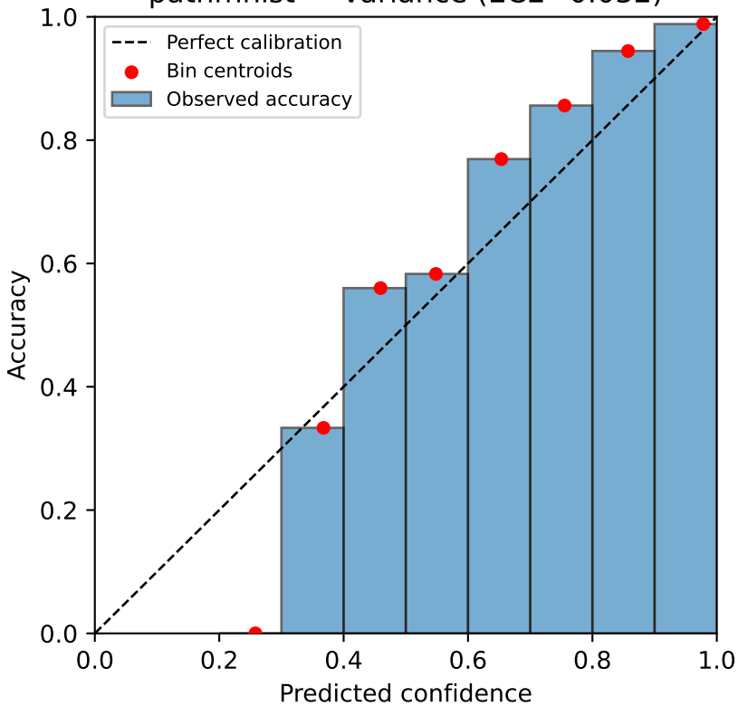
pathmnist — variance (ECE=0.032)
