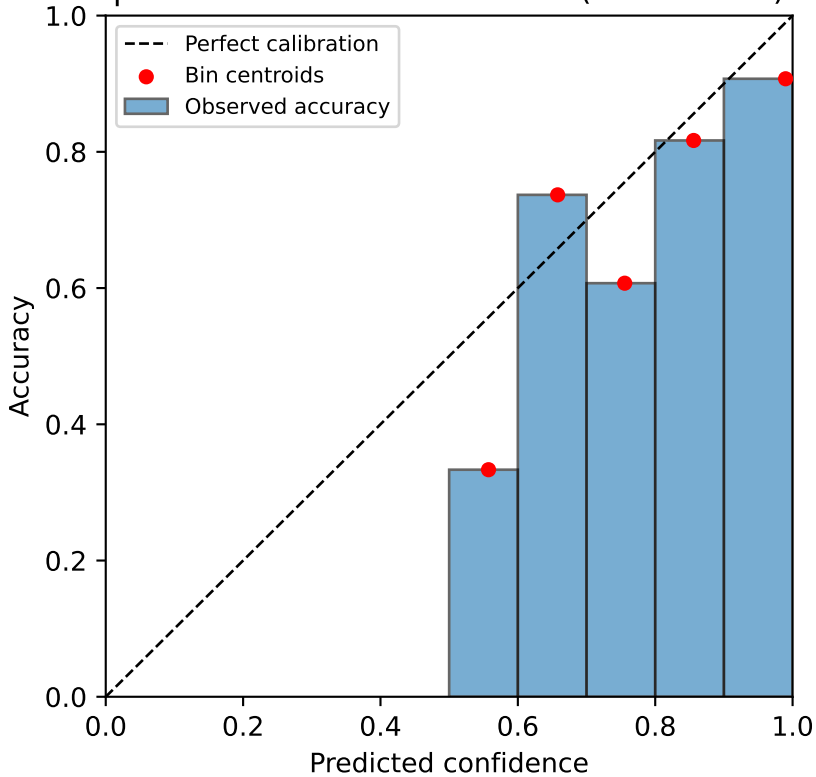
pneumoniarnist — baseline (ECE=0.086)
