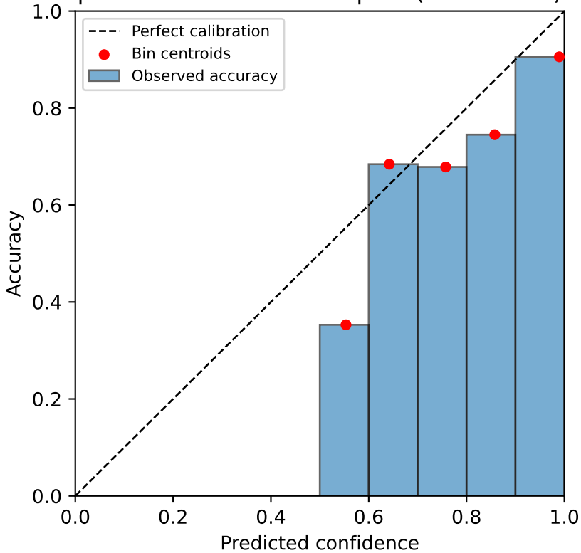
pneumoniarnist — maxprob (ECE=0.088)
