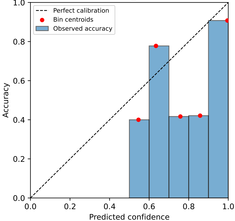
pneumoniamnist — mc_dropout (ECE=0.105)
