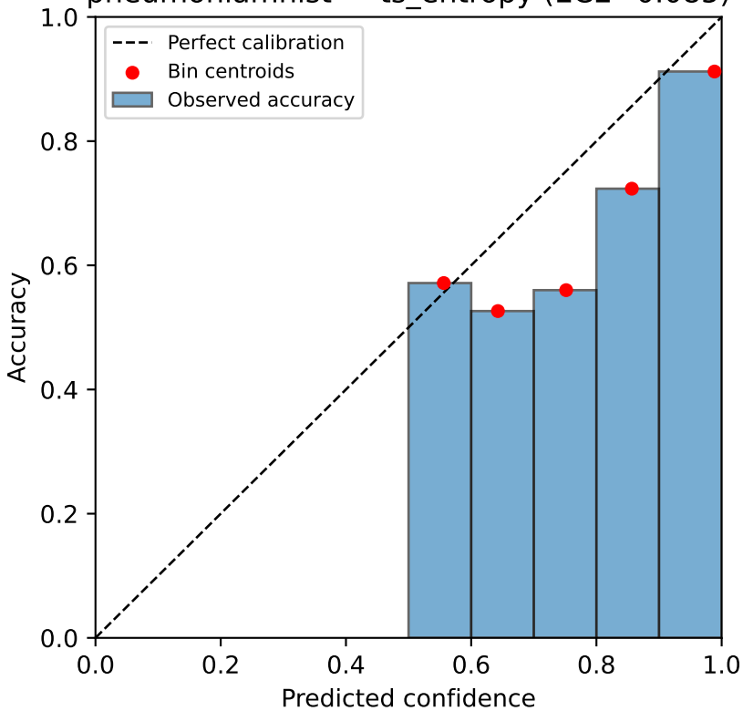
pneumoniamnist — ts_entropy (ECE=0.085)
