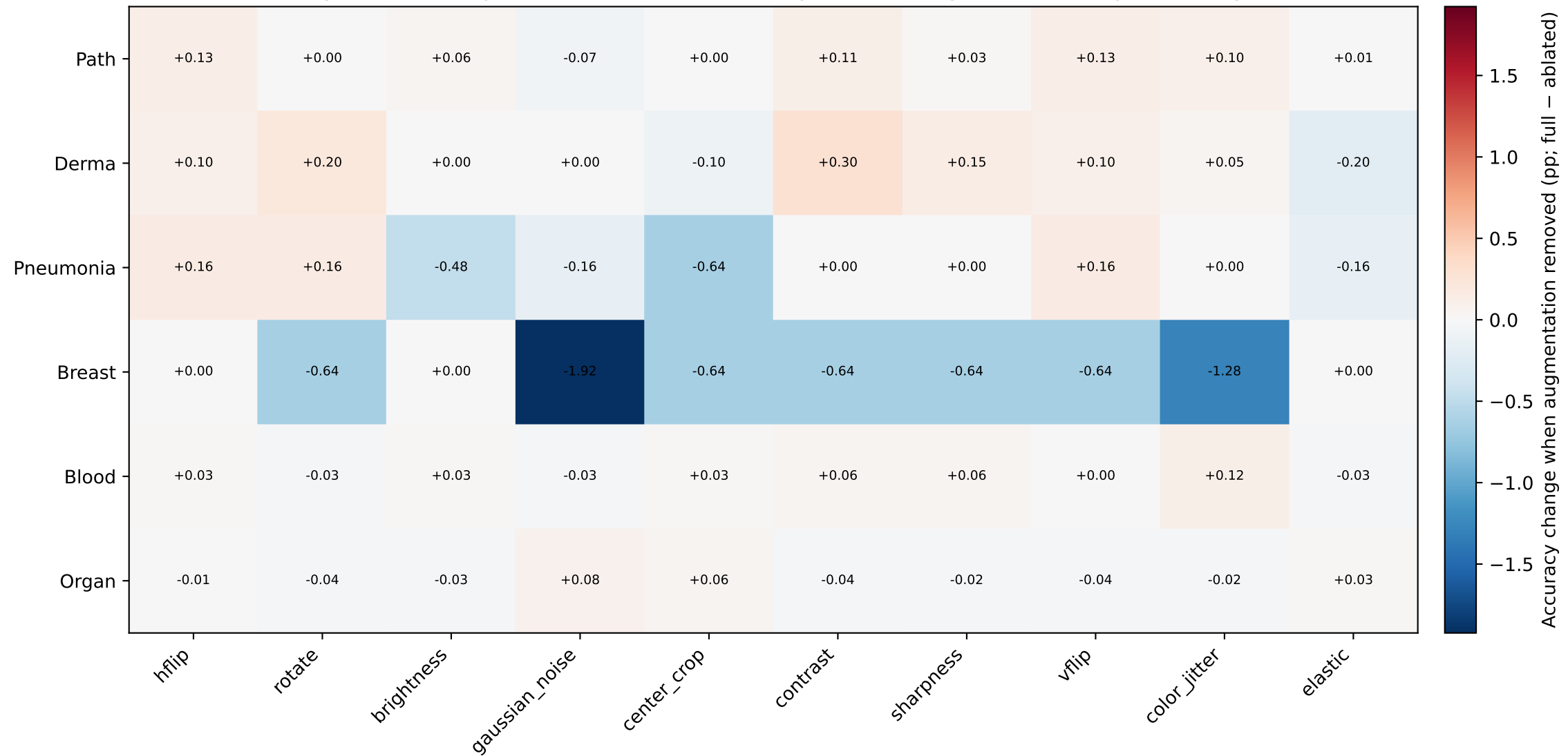
Augmentation importance — EfficientNet-B0 (positive = augmentation helps accuracy)
