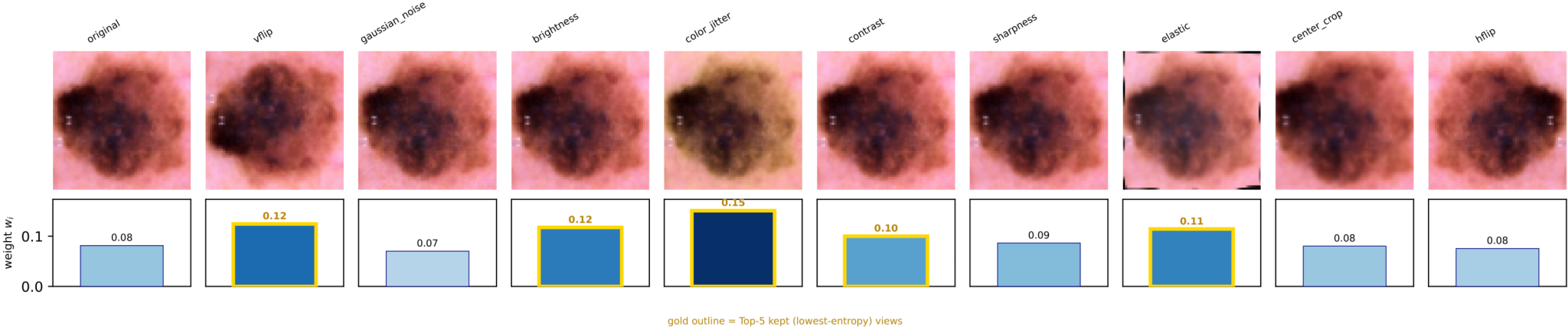
Augmentation Confidence Strip — DermaMNIST (Dermatoscope) - Sample 6 (idx=1252)
